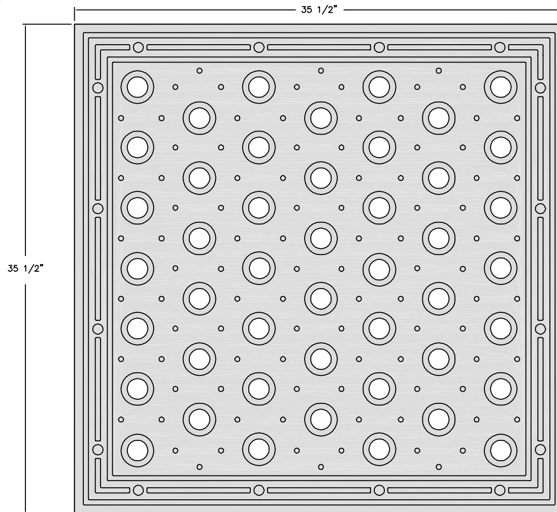
PLAN VIEW
